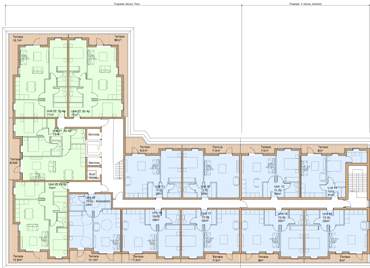
SECOND FLOOR LAYOUT Scale 1:100
